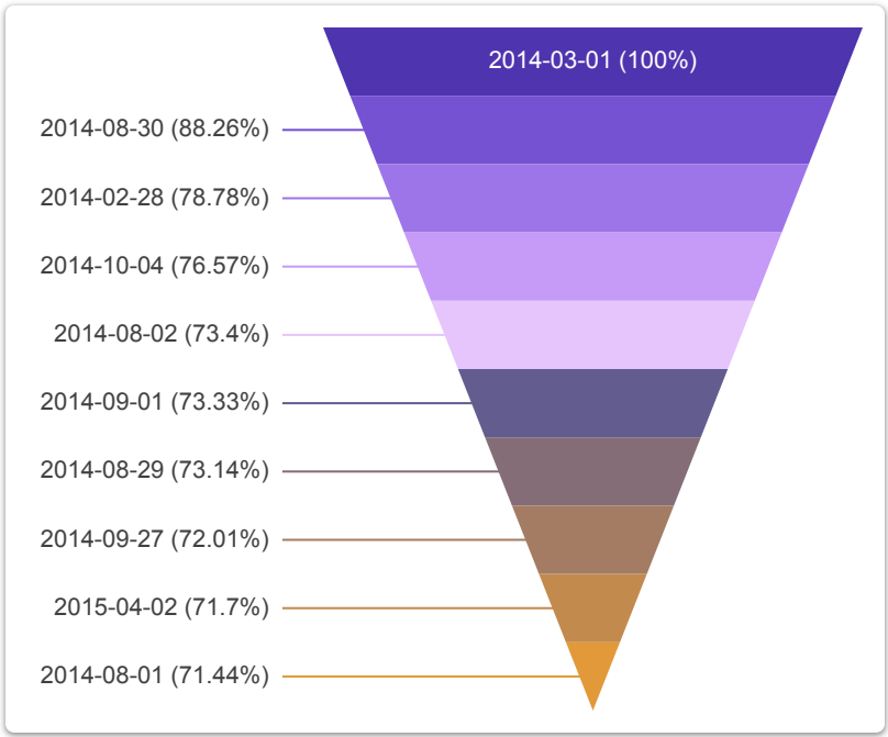
Quantity_Sold Funnel
